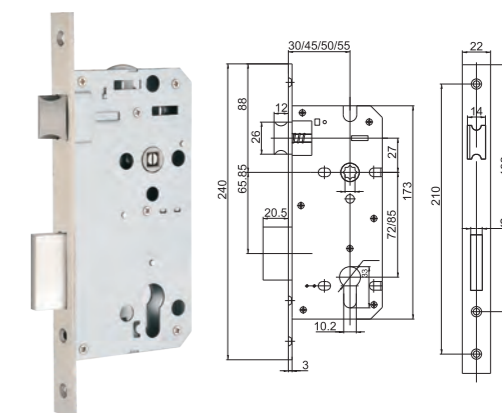
Standard mortise 6085/6072 panic release
